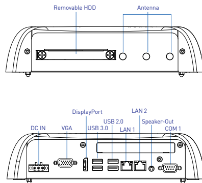
Rear I/O
