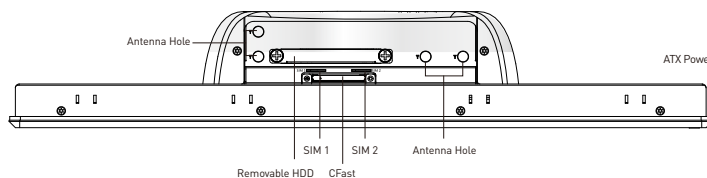
Front I/O
