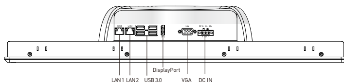
Rear I/O
