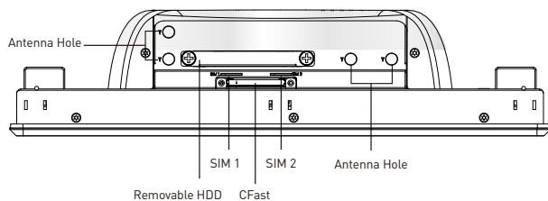
Front I/O
