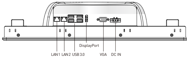
Rear I/O
