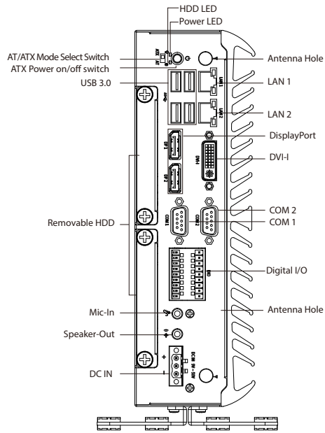
Front Panel
