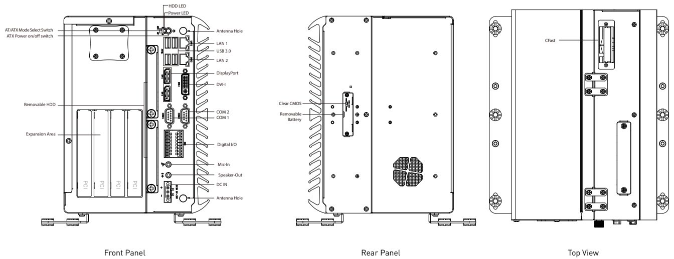
Front Panel
