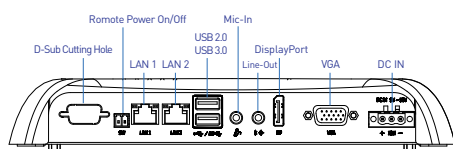
Rear I/O
