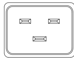
IEC60320 C20
