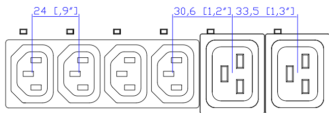
VIEW B
