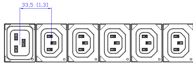
VIEW B
