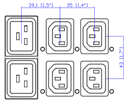
VIEW B
