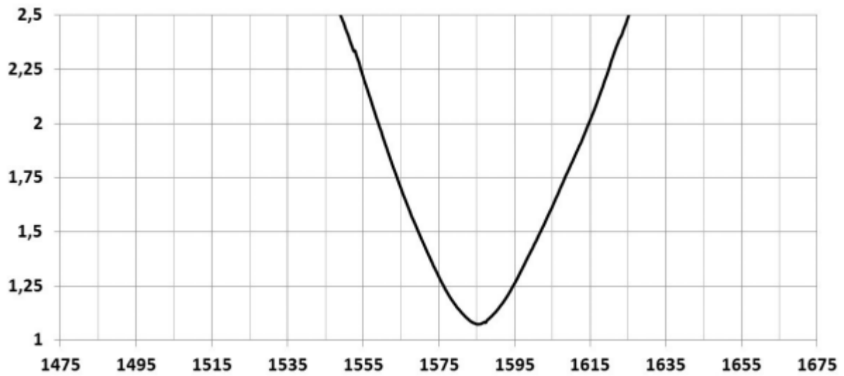
Antenna VSWR
