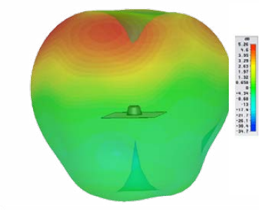
Typical 3D Pattern - Element 2 700MHz
