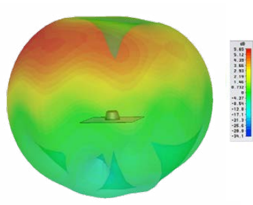
Typical 3D Pattern - Element 2 800MHz
