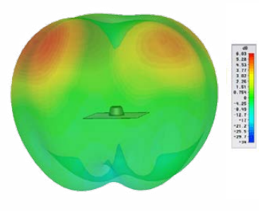
Typical 3D Pattern - Element 2 900MHz
