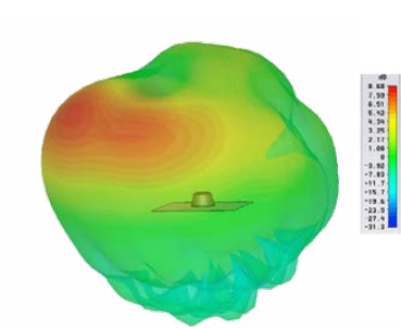
Typical 3D Pattern - Element 2 2000MHz
