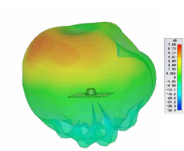
Typical 3D Pattern - Element 2 1800MHz
