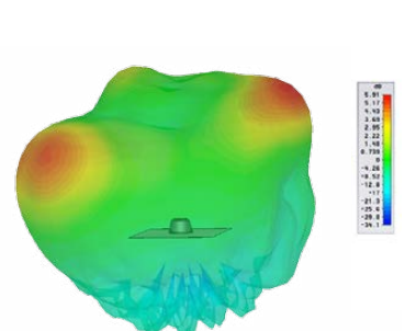
Typical 3D Pattern - Element 2 2600MHz
