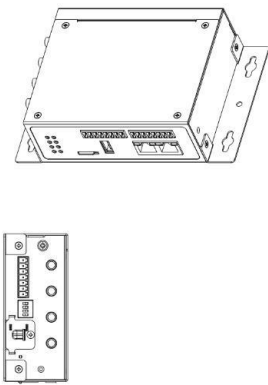
IG502-IO Wall hanging mounting B*
