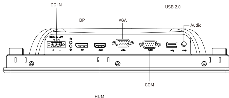
Rear I/O
