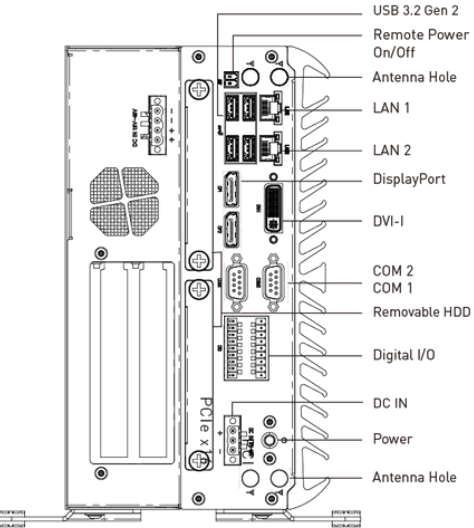
Front Panel
