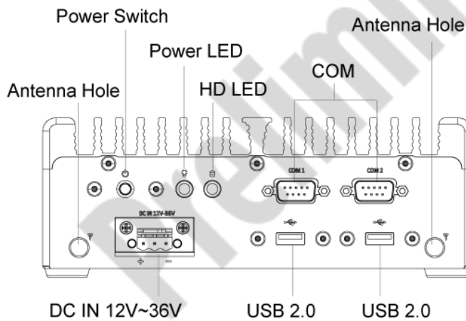
Rear Panel
