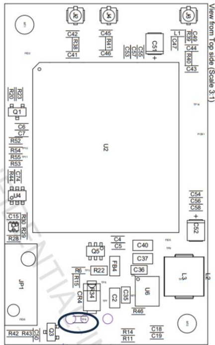
Rev D showing hand placed resistor
